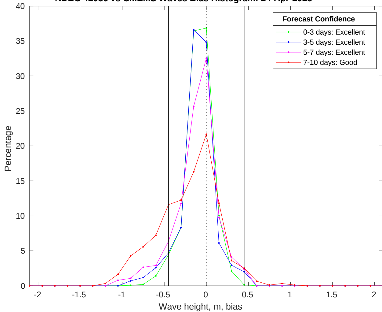
NDBC 42036 vs CMEMS Waves Bias Histogram: 24-Apr-2025
