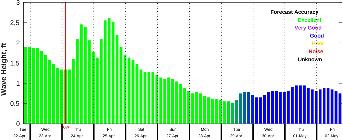
CMEMS Wave Forecast for NDBC 42036 from 22-Apr-2025 19:00:00 to 02-May-2025 19:00:00
