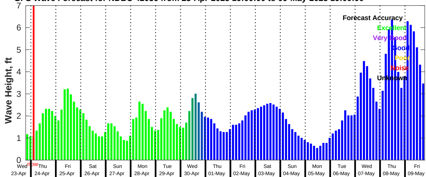
GFS Wave Forecast for NDBC 42036 from 23-Apr-2025 19:00:00 to 09-May-2025 19:00:00
