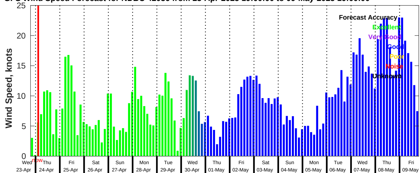
GFS Wind Speed Forecast for NDBC 42036 from 23-Apr-2025 19:00:00 to 09-May-2025 19:00:00
