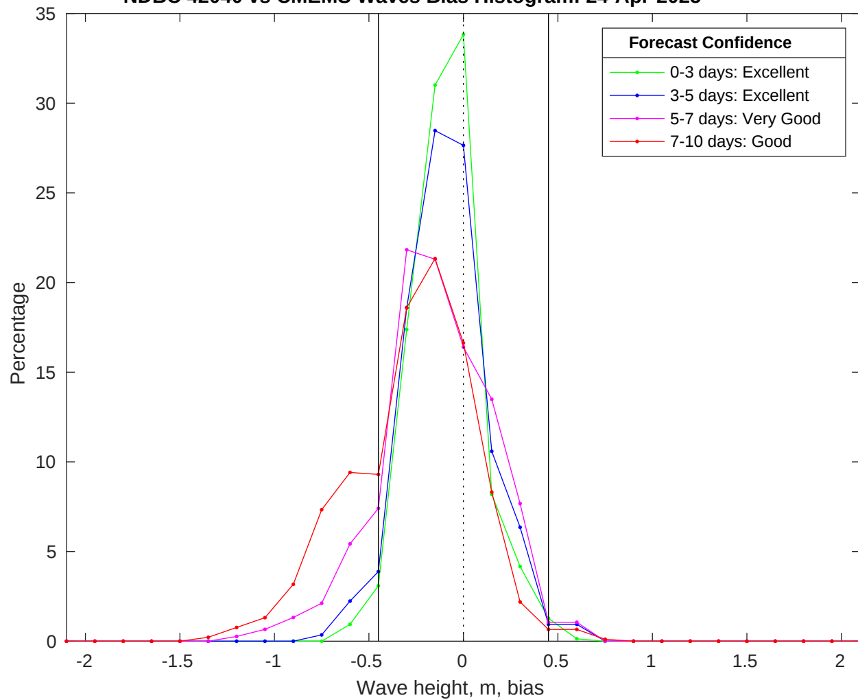
NDBC 42040 vs CMEMS Waves Bias Histogram: 24-Apr-2025
