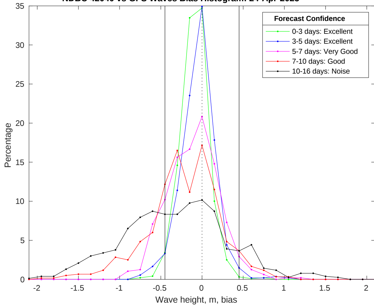
NDBC 42040 vs GFS Waves Bias Histogram: 24-Apr-2025
