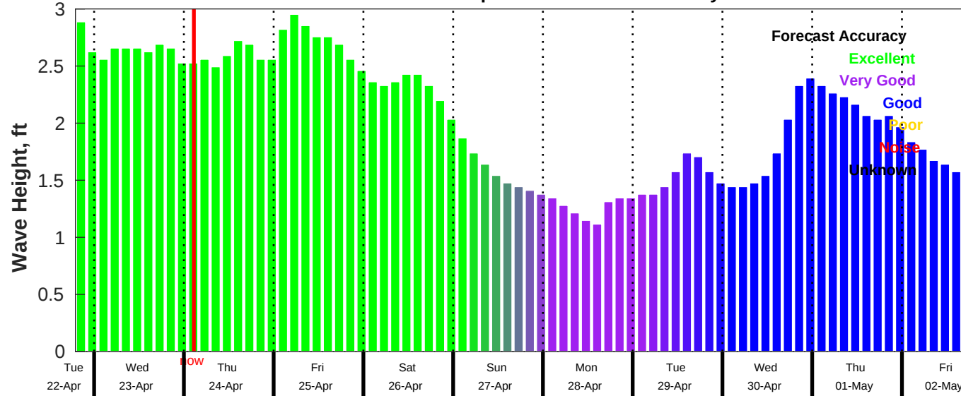
CMEMS Wave Forecast for NDBC 42040 from 22-Apr-2025 19:00:00 to 02-May-2025 19:00:00
