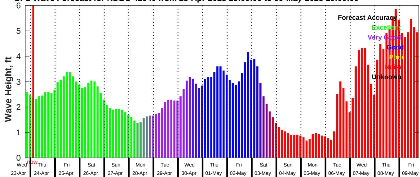
GFS Wave Forecast for NDBC 42040 from 23-Apr-2025 19:00:00 to 09-May-2025 19:00:00
