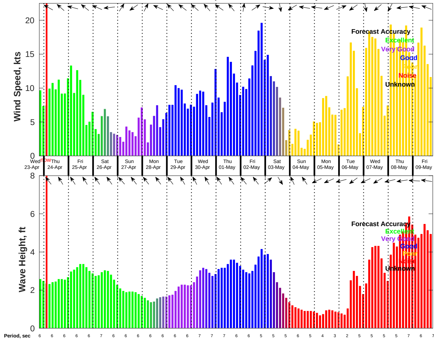
Wind & Wave Forecast for NDBC 42040 from 23-Apr-2025 19:00:00 to 09-May-2025 19:00:00
