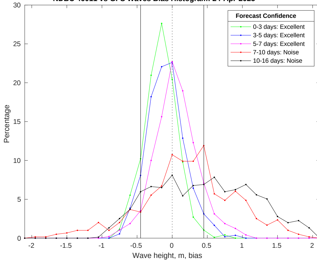
NDBC 46011 vs GFS Waves Bias Histogram: 24-Apr-2025
