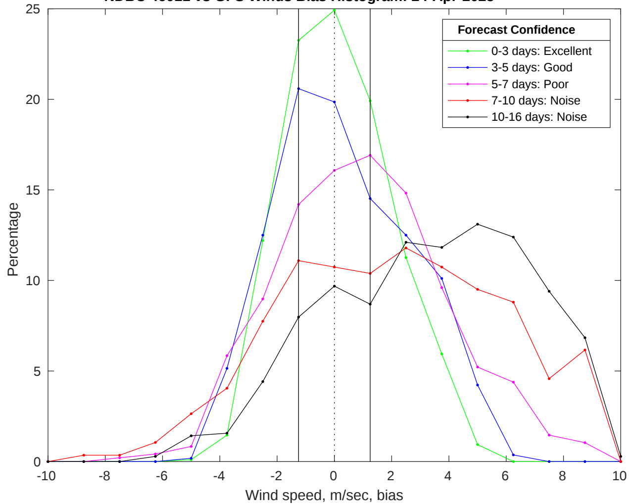
NDBC 46011 vs GFS Winds Bias Histogram: 24-Apr-2025
