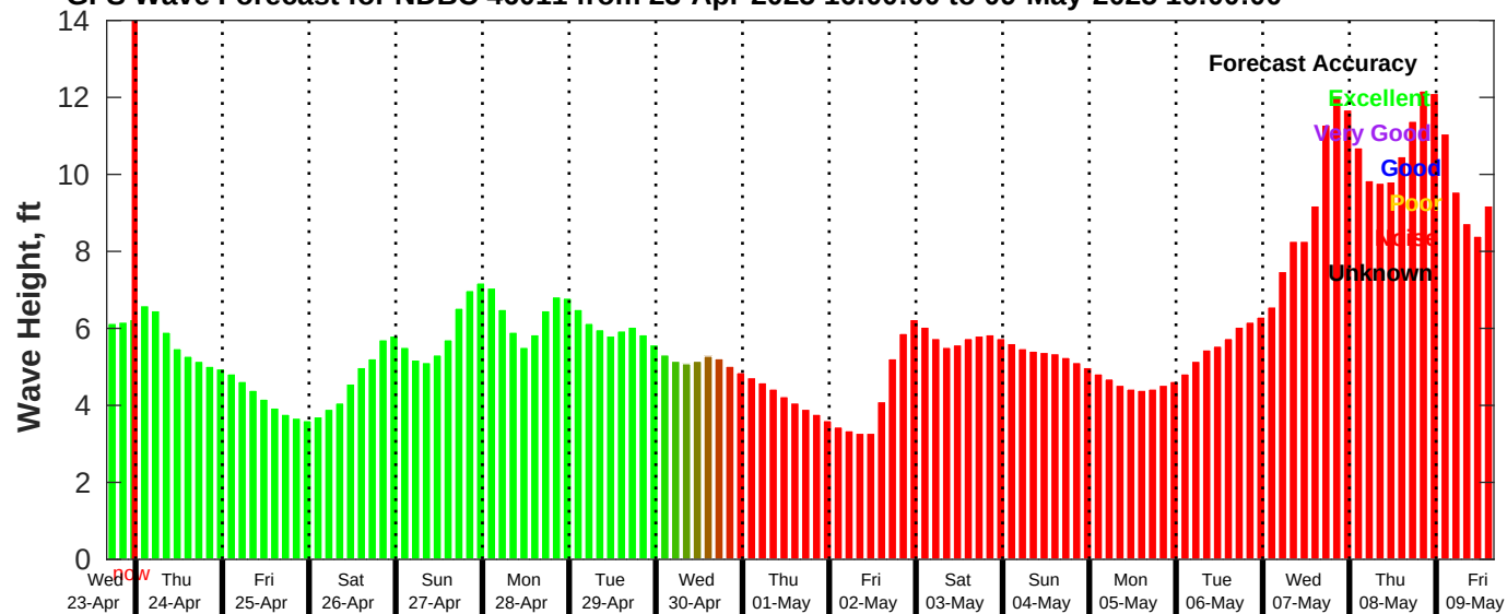
GFS Wave Forecast for NDBC 46011 from 23-Apr-2025 16:00:00 to 09-May-2025 16:00:00
