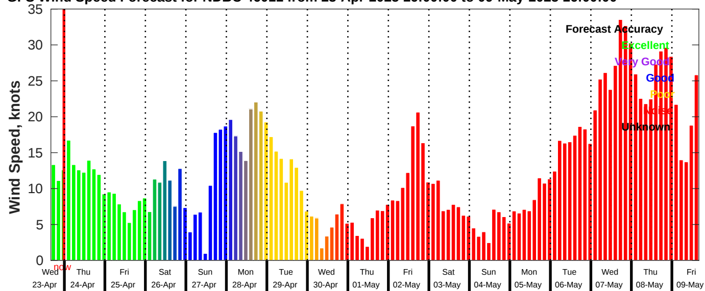
GFS Wind Speed Forecast for NDBC 46011 from 23-Apr-2025 16:00:00 to 09-May-2025 16:00:00
