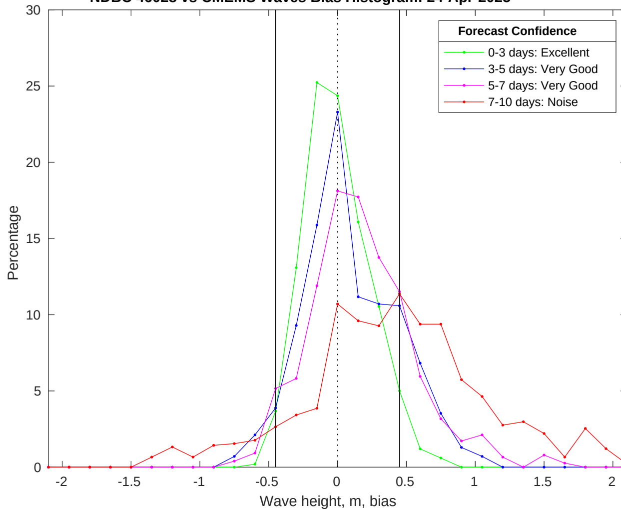
NDBC 46028 vs CMEMS Waves Bias Histogram: 24-Apr-2025
