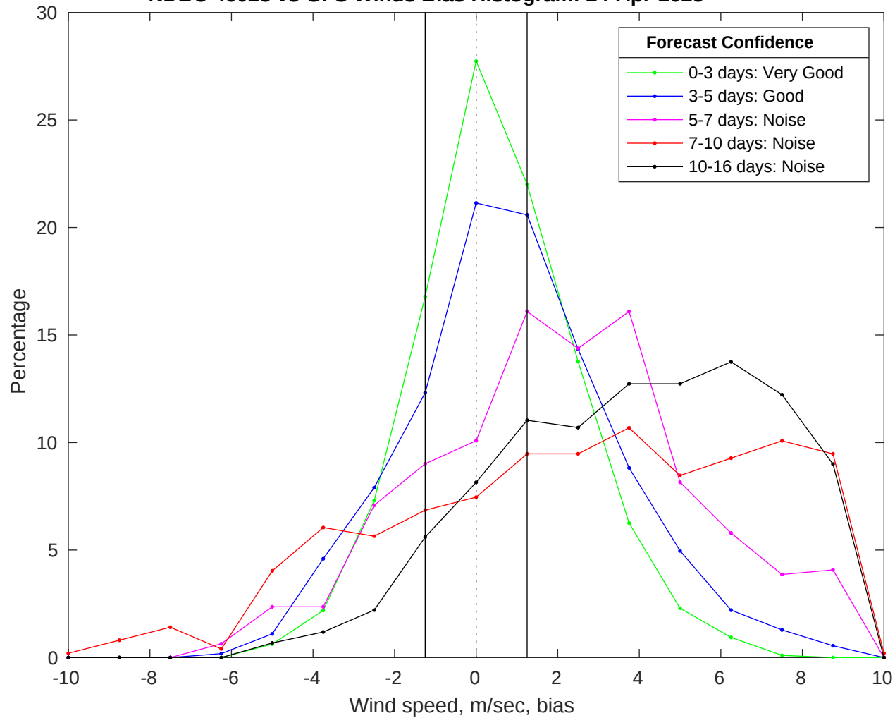
NDBC 46028 vs GFS Winds Bias Histogram: 24-Apr-2025
