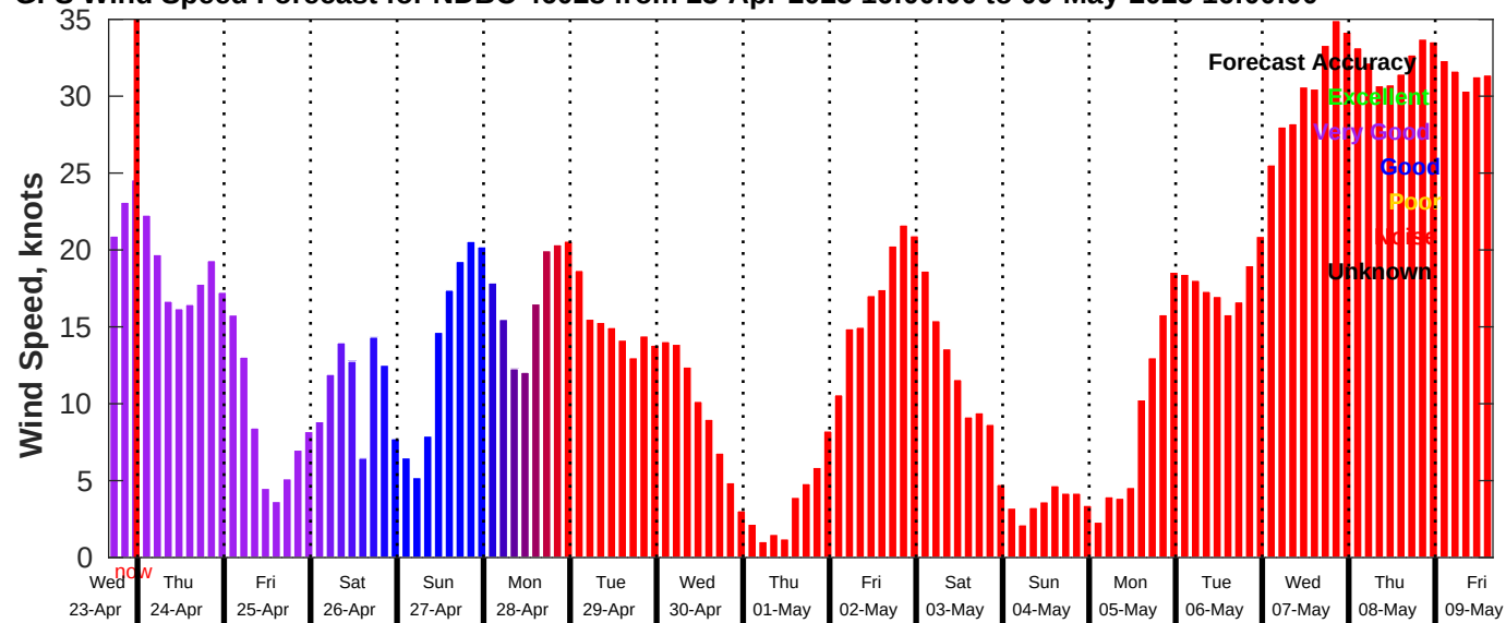
GFS Wind Speed Forecast for NDBC 46028 from 23-Apr-2025 16:00:00 to 09-May-2025 16:00:00
