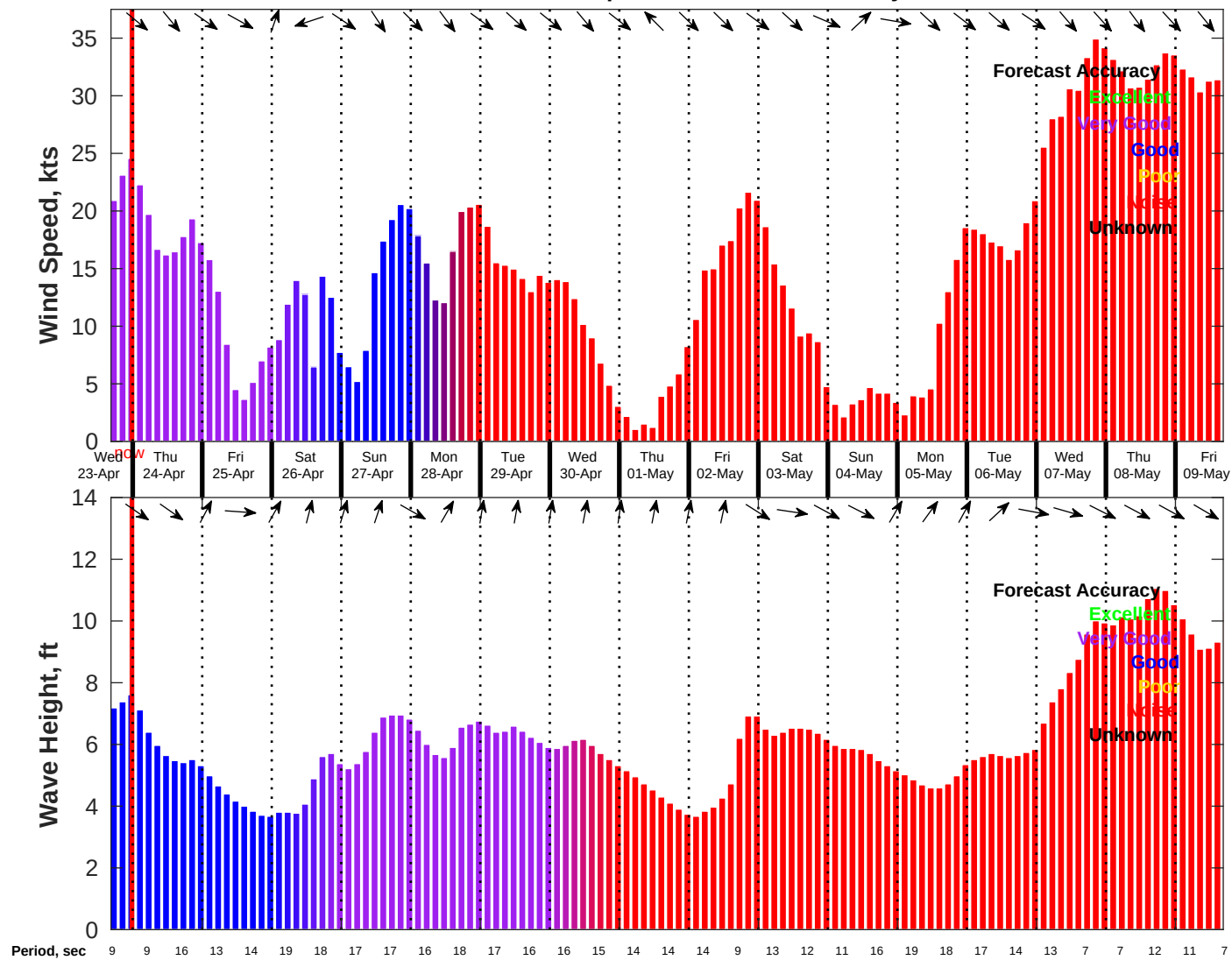
Wind & Wave Forecast for NDBC 46028 from 23-Apr-2025 16:00:00 to 09-May-2025 16:00:00
