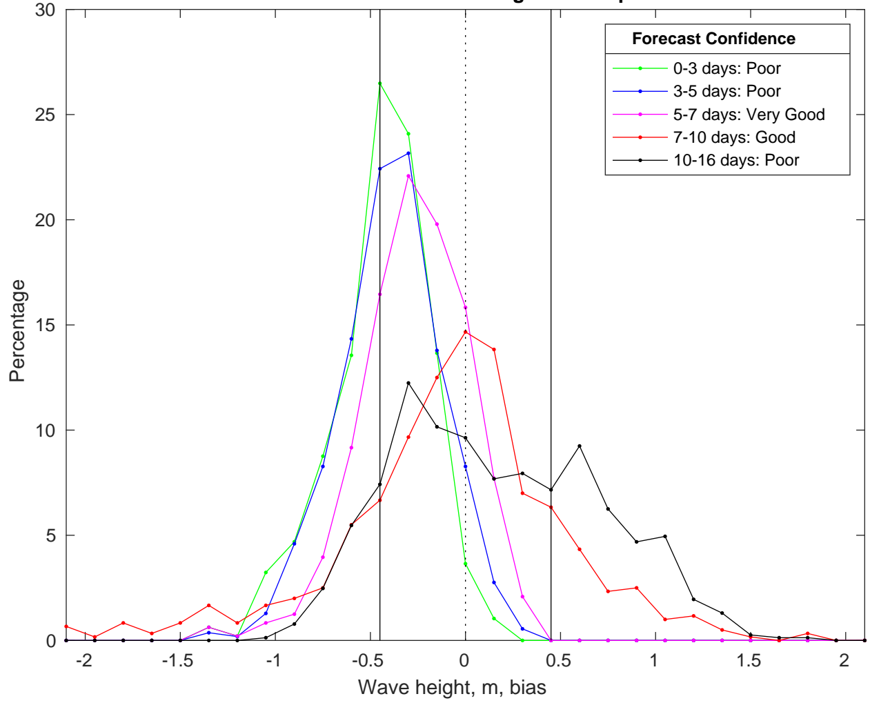
NDBC 46054 vs GFS Waves Bias Histogram: 24-Apr-2025
