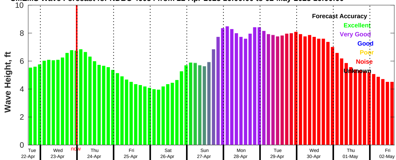
CMEMS Wave Forecast for NDBC 46054 from 22-Apr-2025 16:00:00 to 02-May-2025 16:00:00
