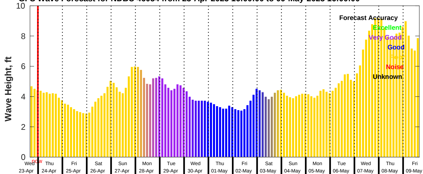
GFS Wave Forecast for NDBC 46054 from 23-Apr-2025 16:00:00 to 09-May-2025 16:00:00
