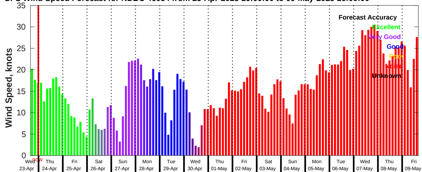
GFS Wind Speed Forecast for NDBC 46054 from 23-Apr-2025 16:00:00 to 09-May-2025 16:00:00
