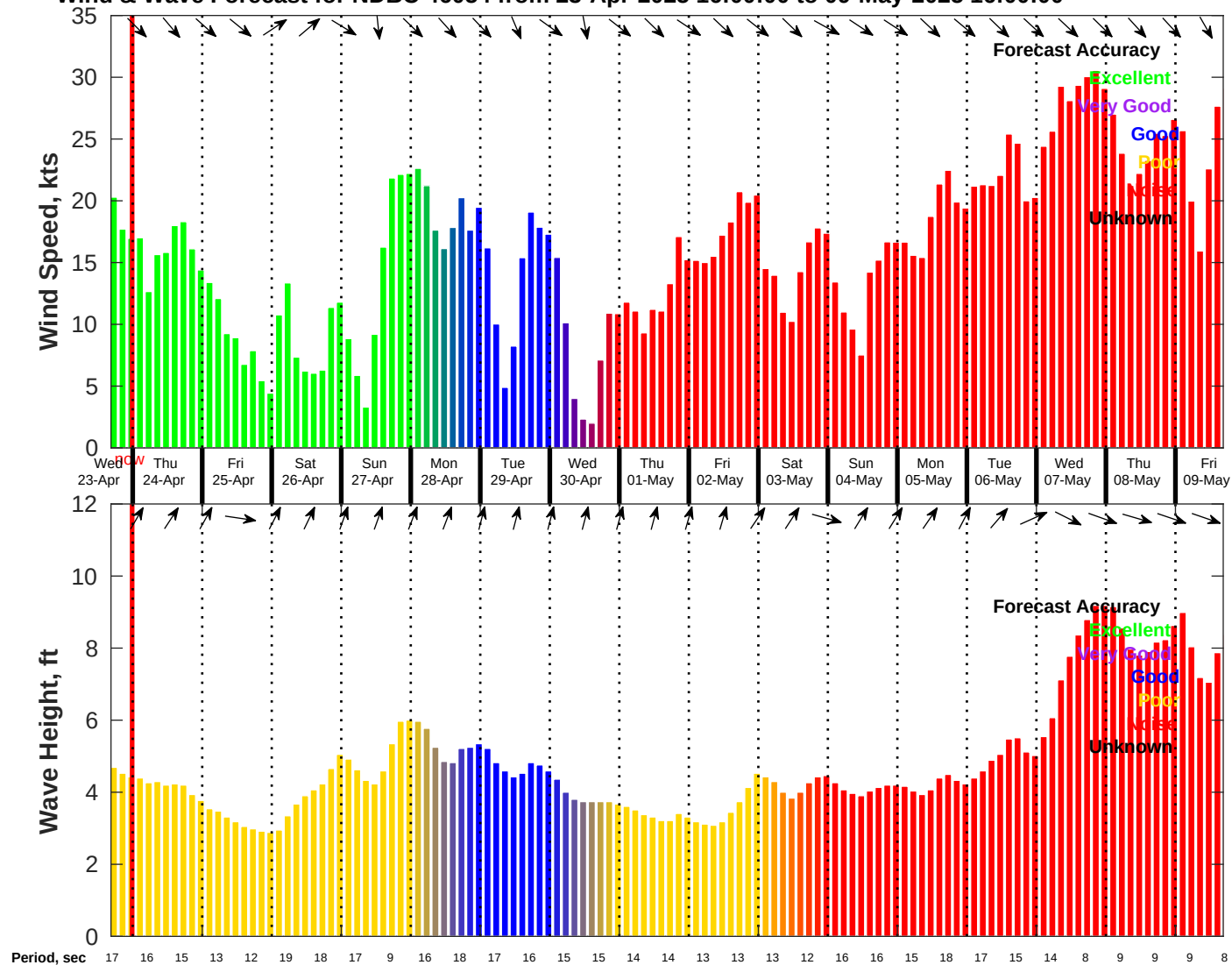
Wind & Wave Forecast for NDBC 46054 from 23-Apr-2025 16:00:00 to 09-May-2025 16:00:00
