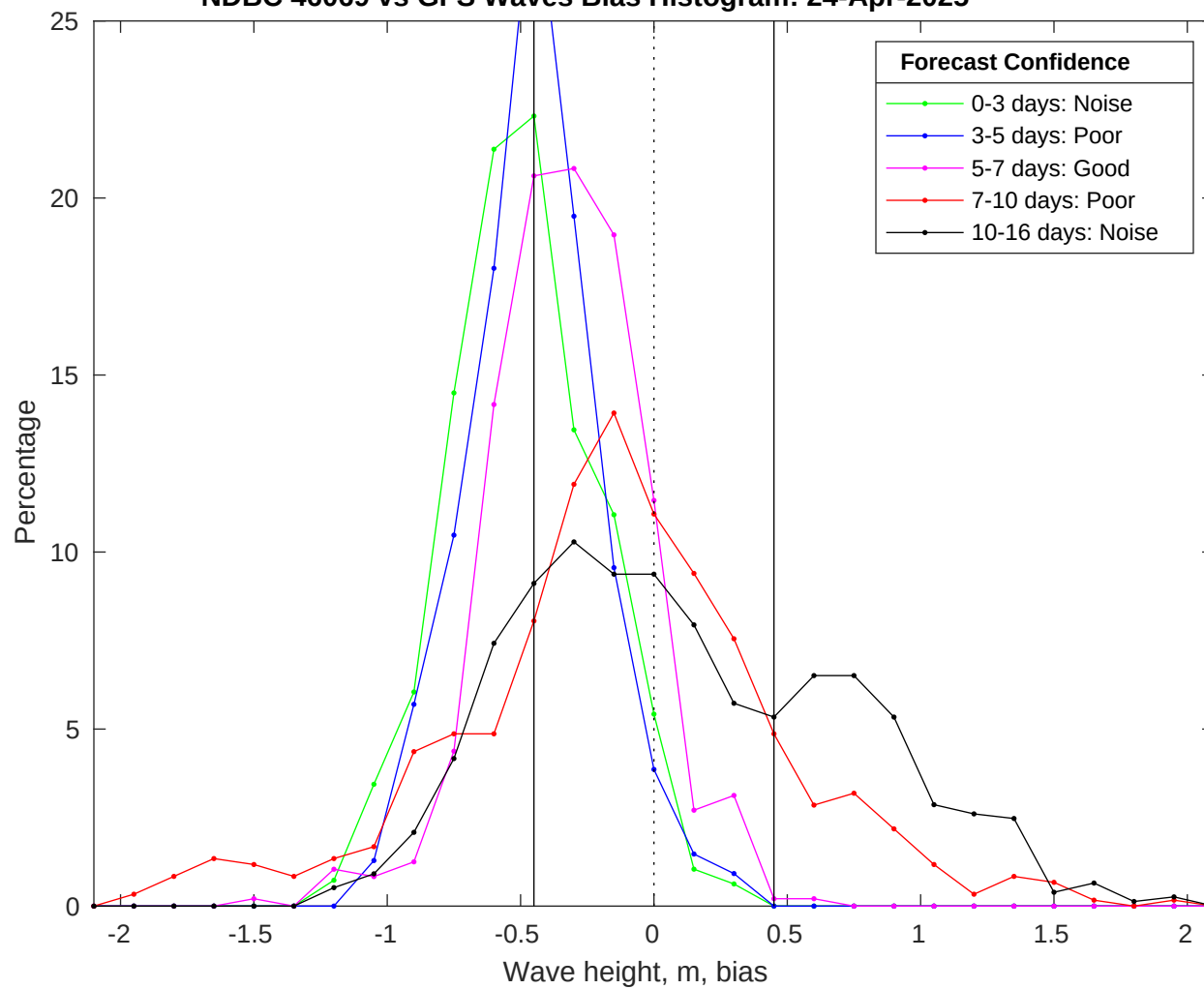
NDBC 46069 vs GFS Waves Bias Histogram: 24-Apr-2025
