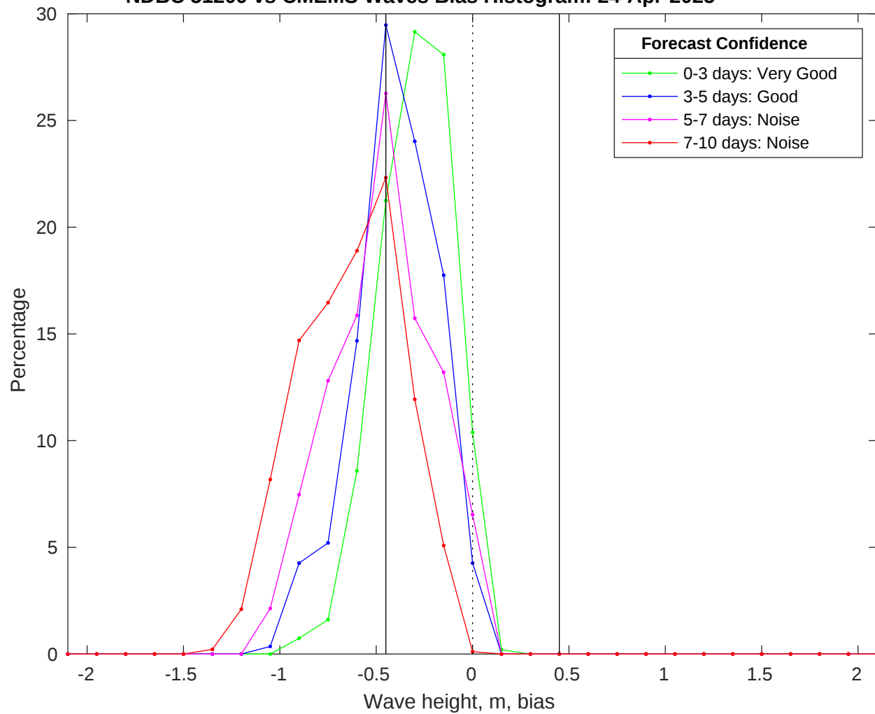
NDBC 51209 vs CMEMS Waves Bias Histogram: 24-Apr-2025
