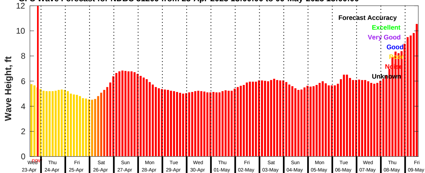
GFS Wave Forecast for NDBC 51209 from 23-Apr-2025 13:00:00 to 09-May-2025 13:00:00
