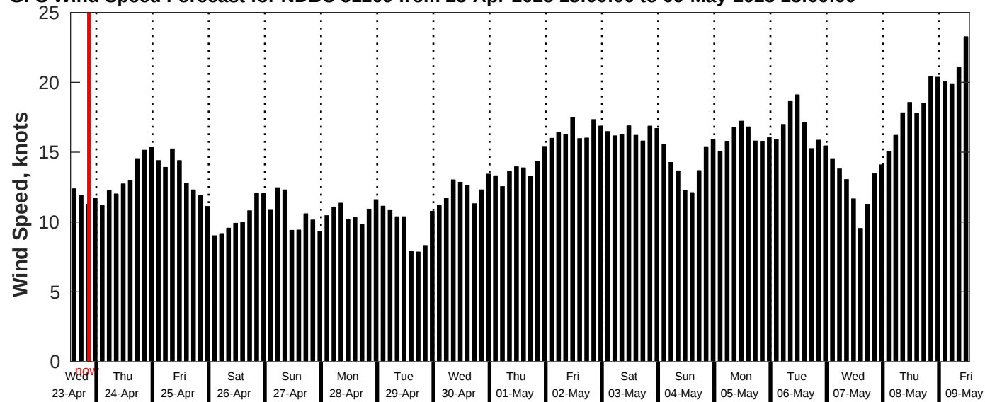
GFS Wind Speed Forecast for NDBC 51209 from 23-Apr-2025 13:00:00 to 09-May-2025 13:00:00
