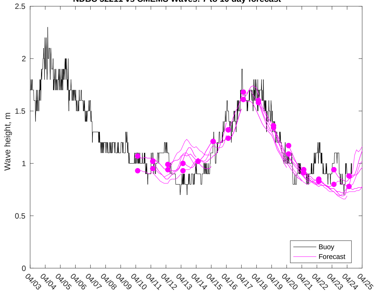
NDBC 52211 vs CMEMS Waves: 7 to 10 day forecast
