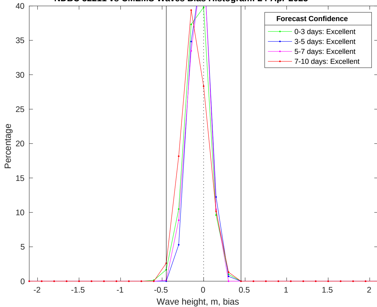
NDBC 52211 vs CMEMS Waves Bias Histogram: 24-Apr-2025
