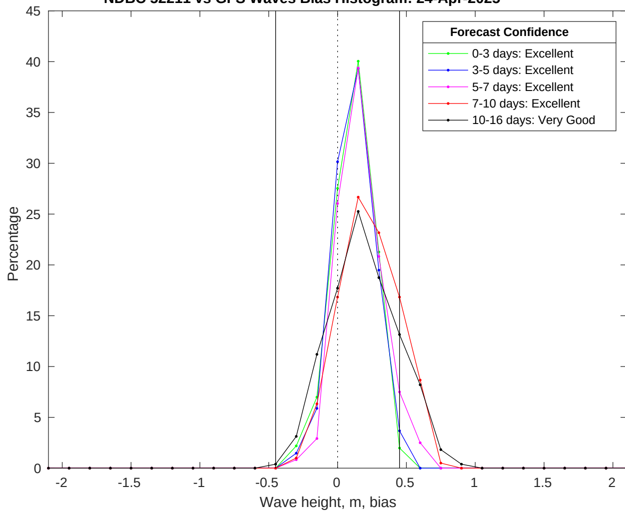
NDBC 52211 vs GFS Waves Bias Histogram: 24-Apr-2025
