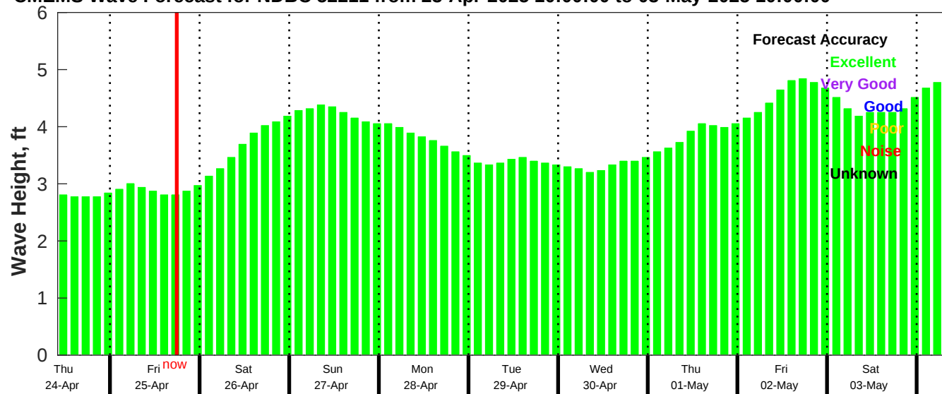
CMEMS Wave Forecast for NDBC 52211 from 23-Apr-2025 10:00:00 to 03-May-2025 10:00:00
