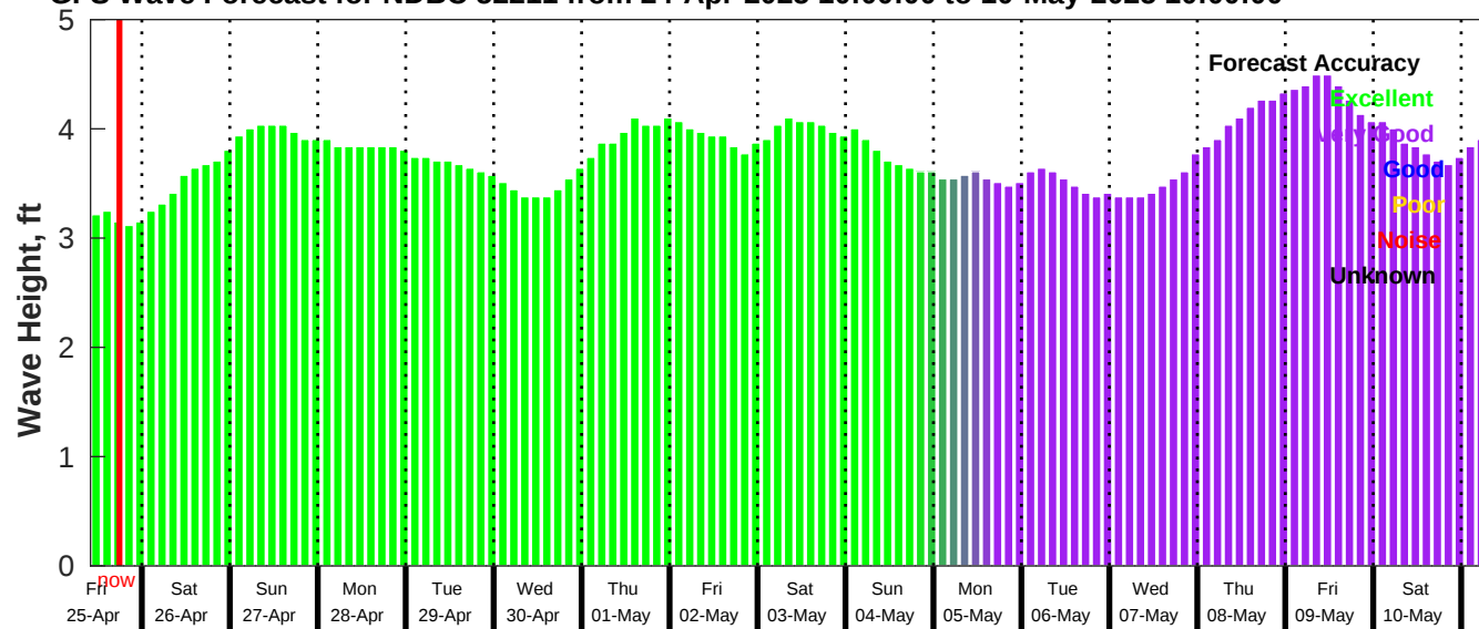
GFS Wave Forecast for NDBC 52211 from 24-Apr-2025 10:00:00 to 10-May-2025 10:00:00
