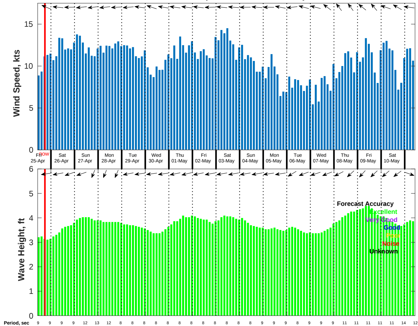
Wind & Wave Forecast for NDBC 52211 from 24-Apr-2025 10:00:00 to 10-May-2025 10:00:00
