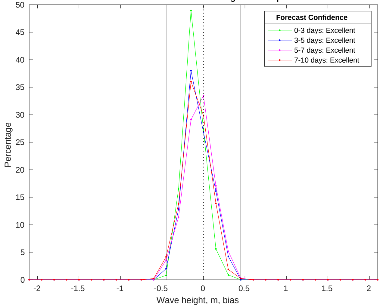
NDBC 52212 vs CMEMS Waves Bias Histogram: 24-Apr-2025
