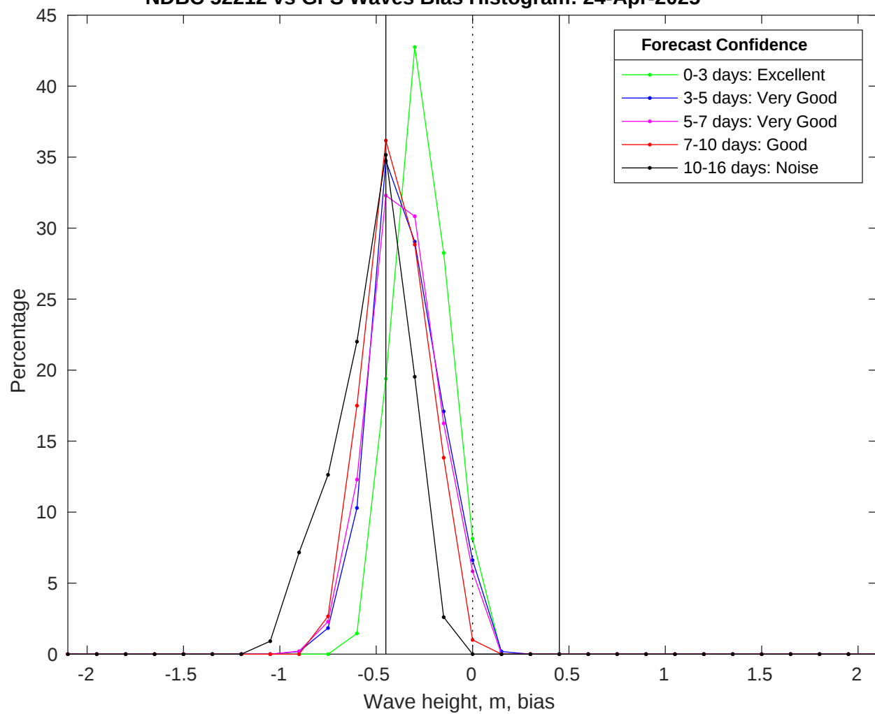
NDBC 52212 vs GFS Waves Bias Histogram: 24-Apr-2025
