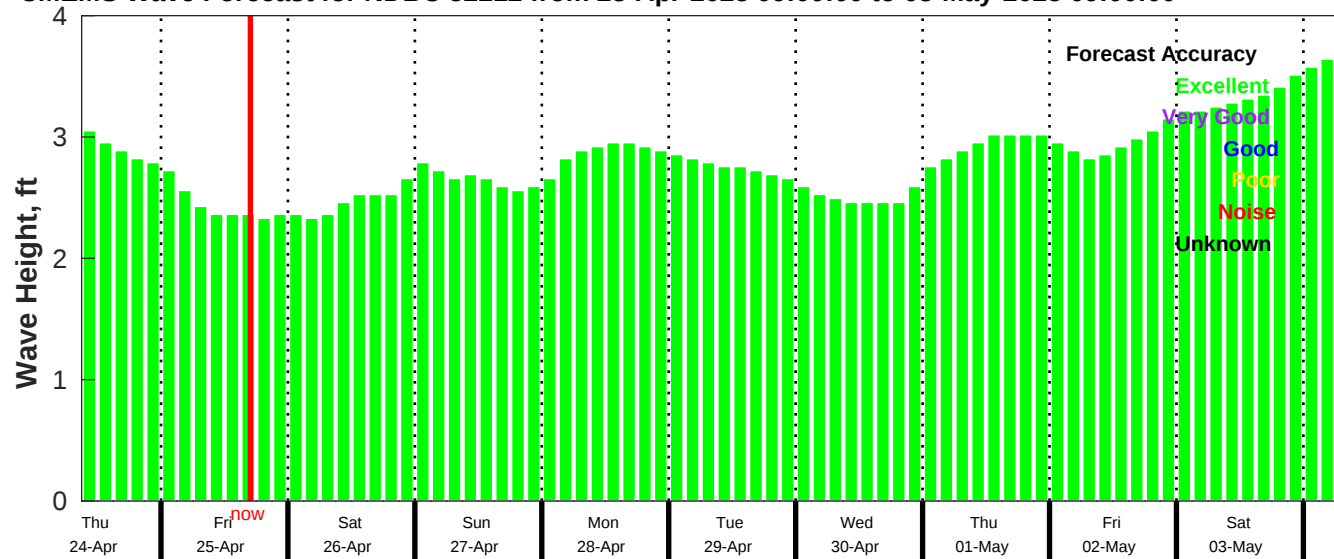
CMEMS Wave Forecast for NDBC 52212 from 23-Apr-2025 09:00:00 to 03-May-2025 09:00:00
