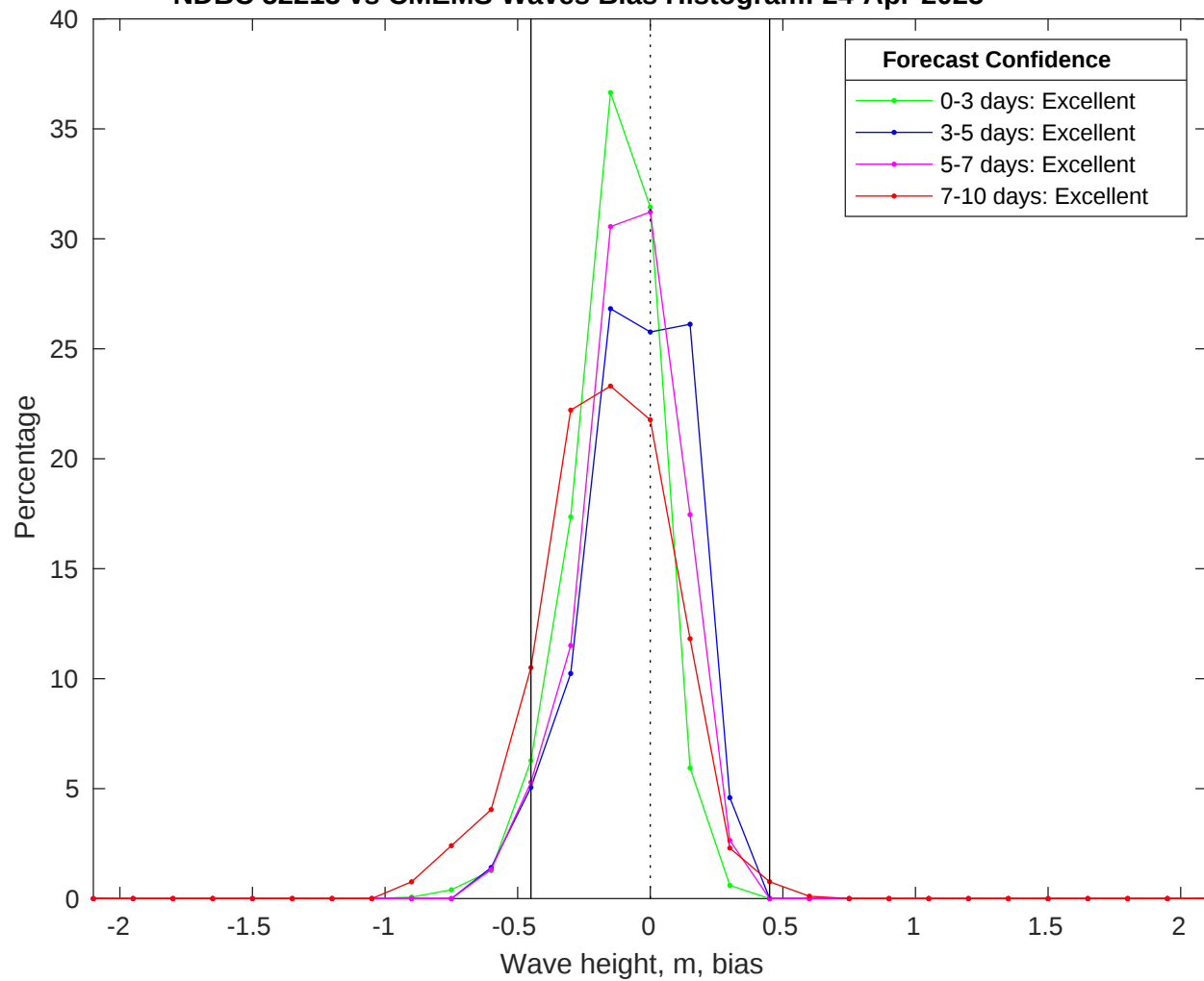
NDBC 52213 vs CMEMS Waves Bias Histogram: 24-Apr-2025
