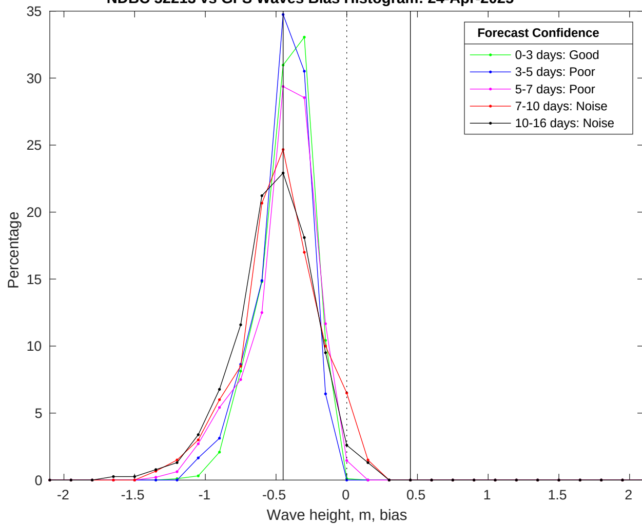
NDBC 52213 vs GFS Waves Bias Histogram: 24-Apr-2025
