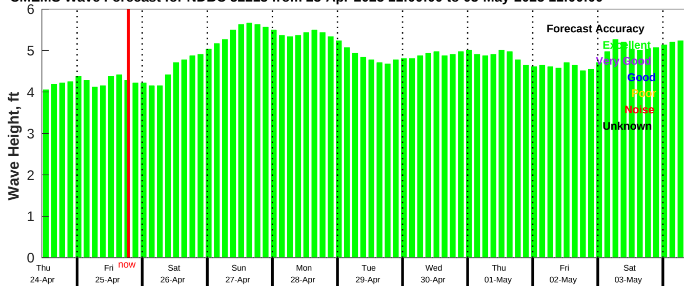
CMEMS Wave Forecast for NDBC 52213 from 23-Apr-2025 11:00:00 to 03-May-2025 11:00:00
