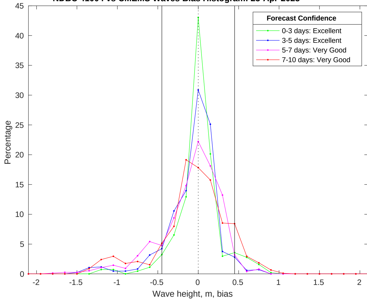
NDBC 41004 vs CMEMS Waves Bias Histogram: 25-Apr-2025
