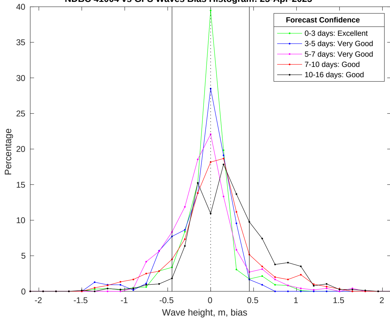
NDBC 41004 vs GFS Waves Bias Histogram: 25-Apr-2025
