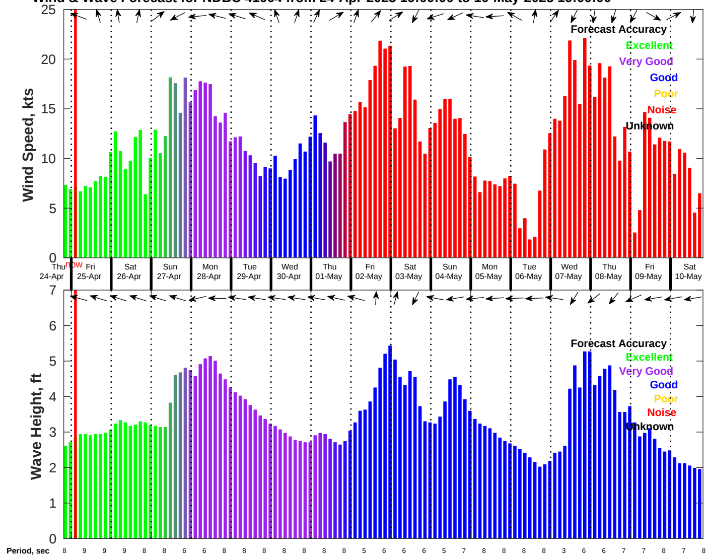
Wind & Wave Forecast for NDBC 41004 from 24-Apr-2025 19:00:00 to 10-May-2025 19:00:00
