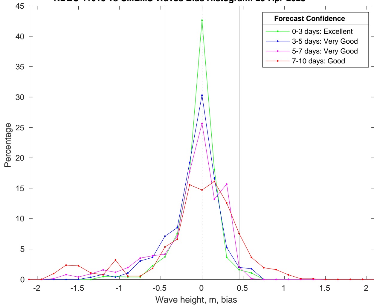
NDBC 41013 vs CMEMS Waves Bias Histogram: 25-Apr-2025
