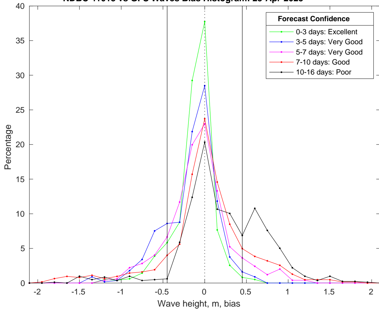
NDBC 41013 vs GFS Waves Bias Histogram: 25-Apr-2025
