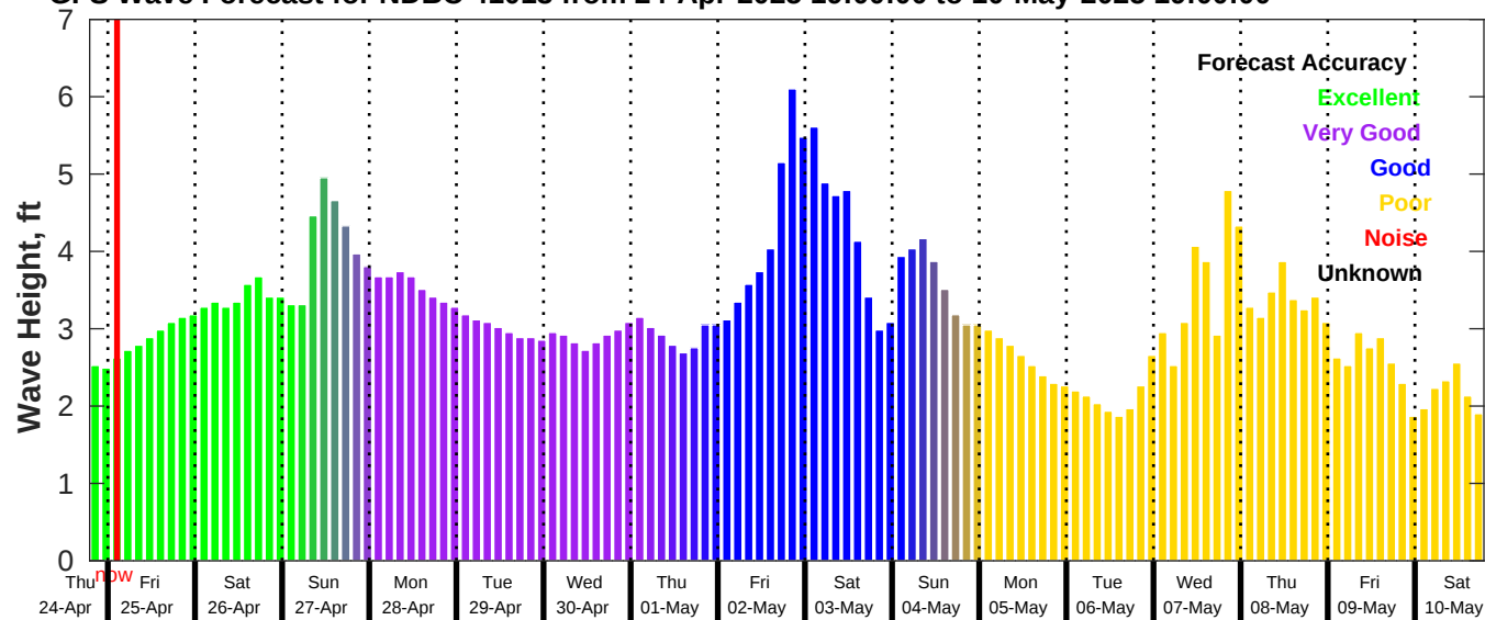
GFS Wave Forecast for NDBC 41013 from 24-Apr-2025 19:00:00 to 10-May-2025 19:00:00
