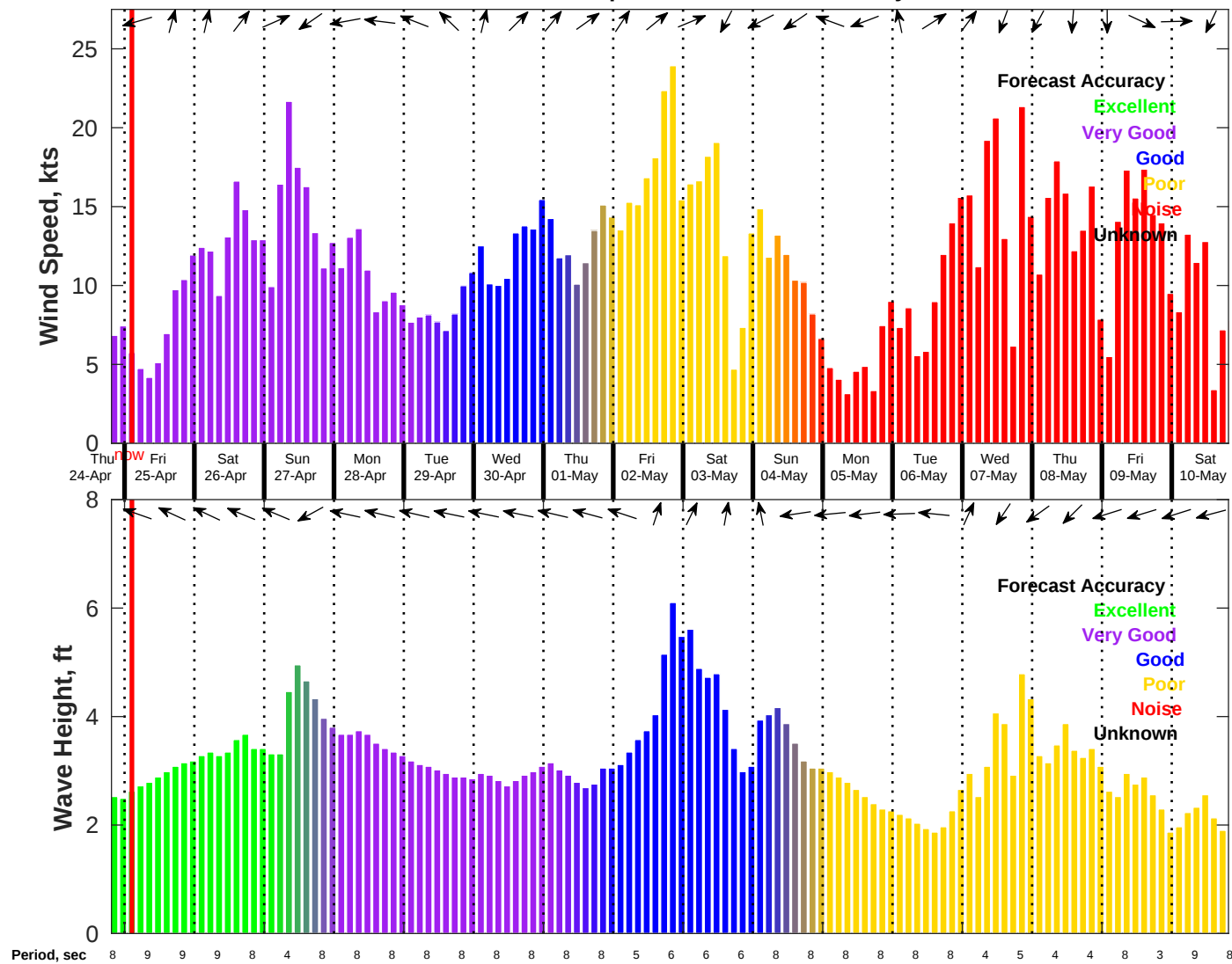
Wind & Wave Forecast for NDBC 41013 from 24-Apr-2025 19:00:00 to 10-May-2025 19:00:00
