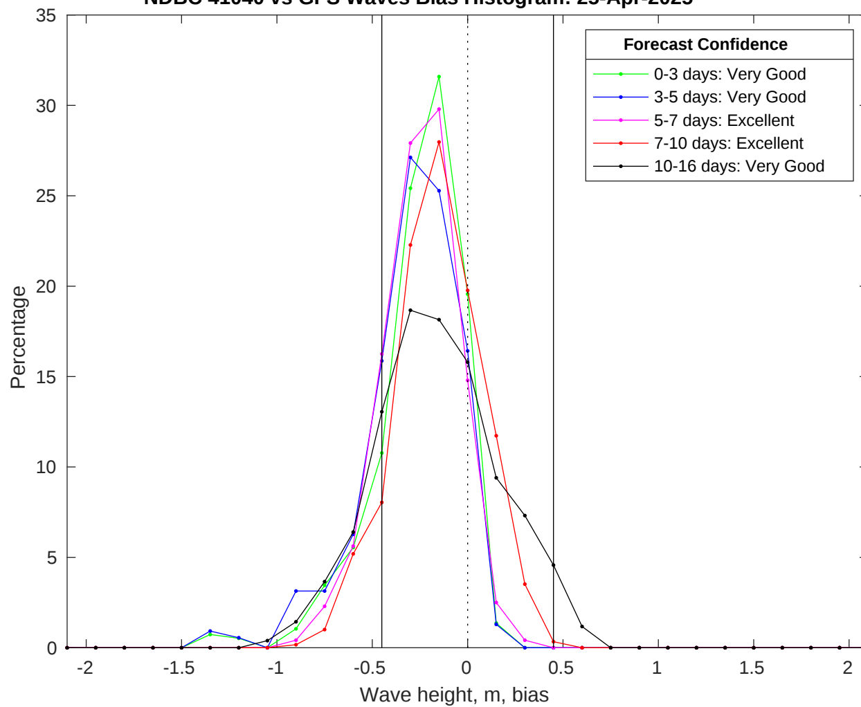
NDBC 41040 vs GFS Waves Bias Histogram: 25-Apr-2025
