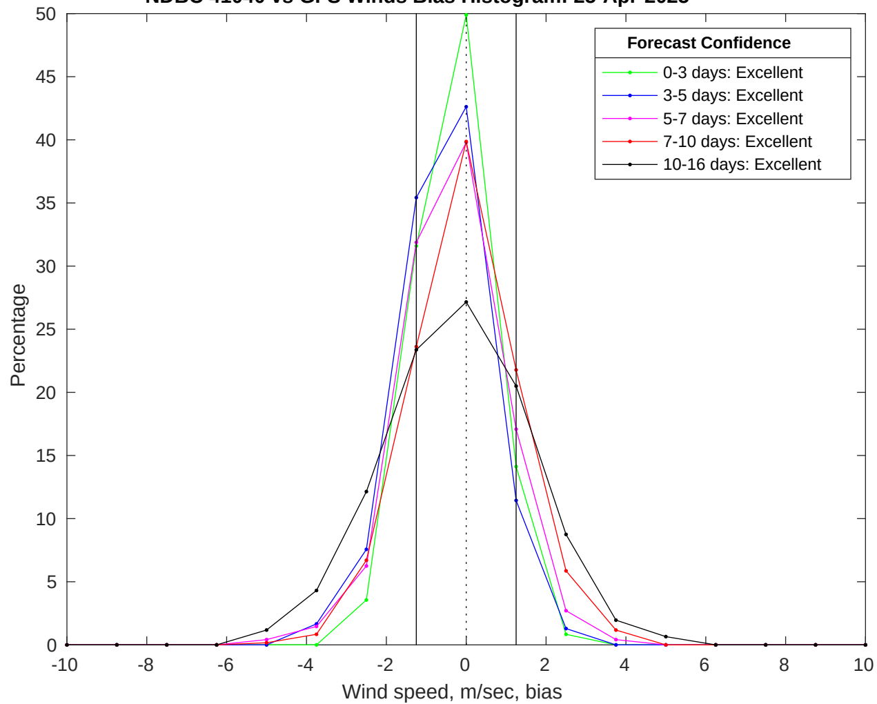
NDBC 41040 vs GFS Winds Bias Histogram: 25-Apr-2025
