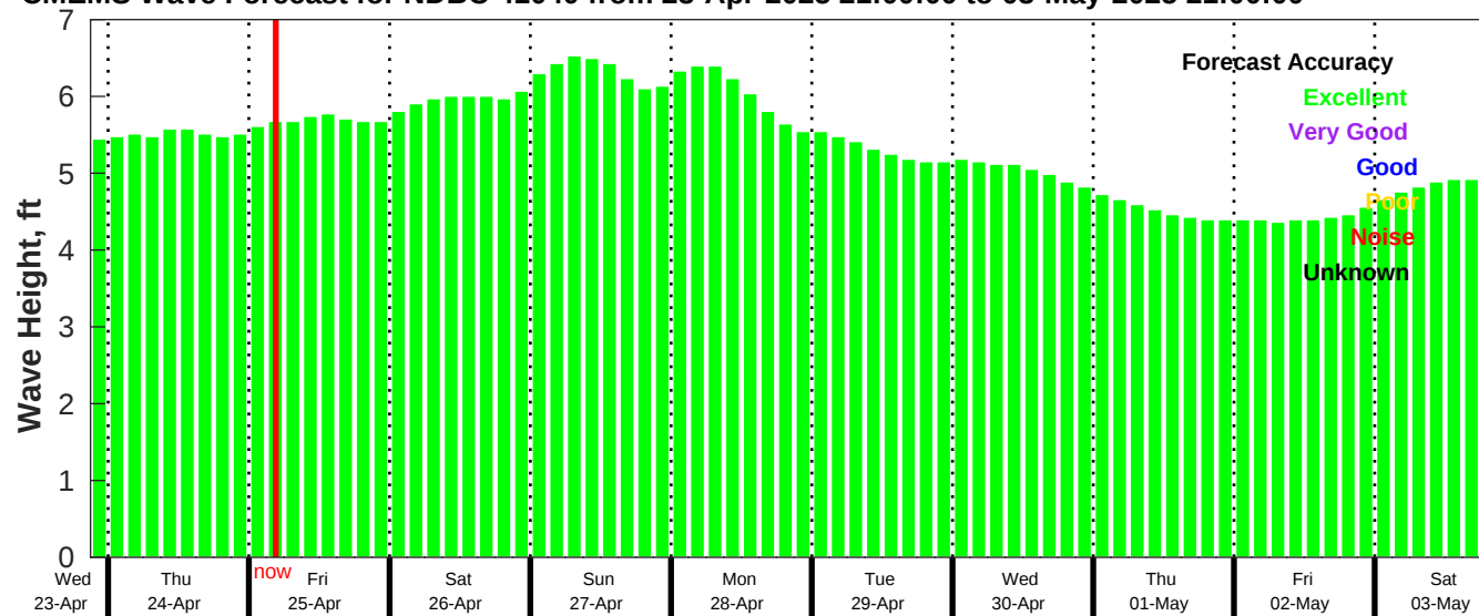
CMEMS Wave Forecast for NDBC 41040 from 23-Apr-2025 21:00:00 to 03-May-2025 21:00:00
