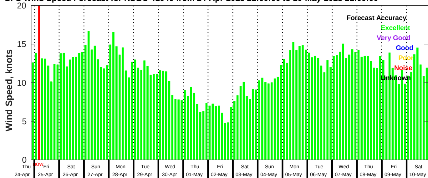
GFS Wind Speed Forecast for NDBC 41040 from 24-Apr-2025 21:00:00 to 10-May-2025 21:00:00
