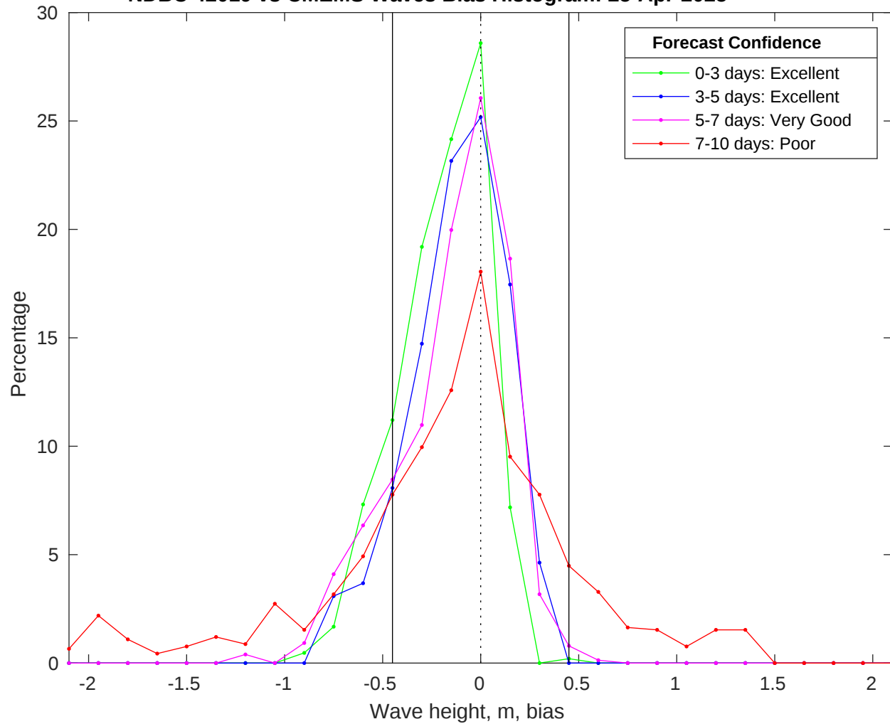
NDBC 42019 vs CMEMS Waves Bias Histogram: 25-Apr-2025
